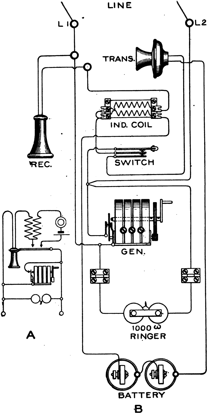
FIG. 84.—Circuit, local battery wall telephone, Dean type.
